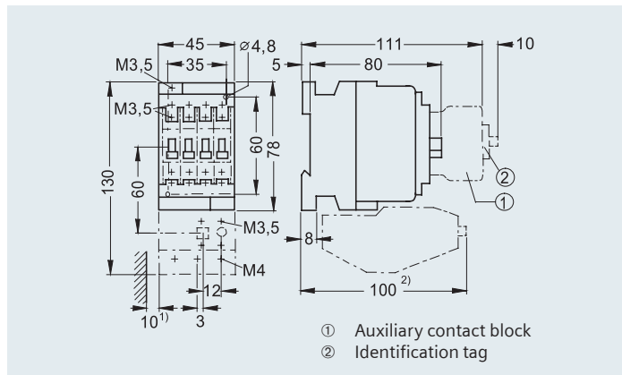
3TF30/31 AC Coil
