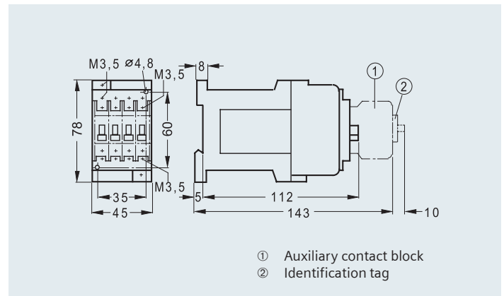
3TF30/31 DC Coil
